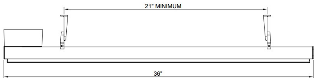
SIDE VIEW
