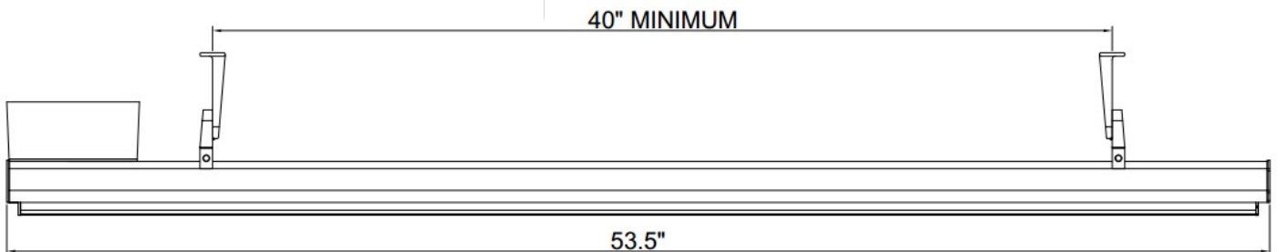
END VIEW
